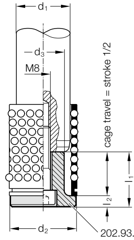
Mounting example
